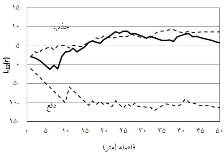
(ELT → ST)
